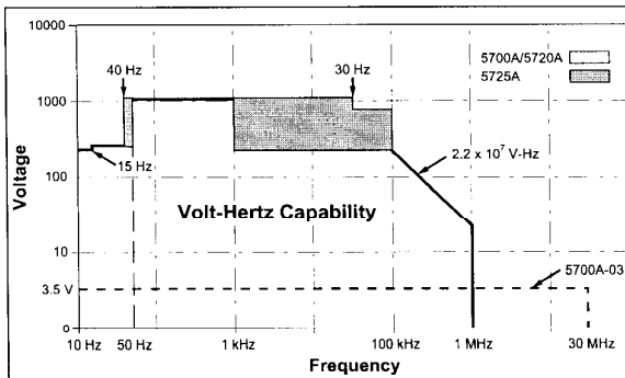
Figure 1-1. Volt-Hertz Capability
